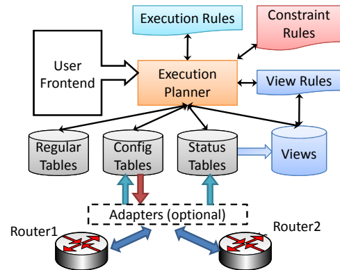
Figure 1: DECOR architecture
