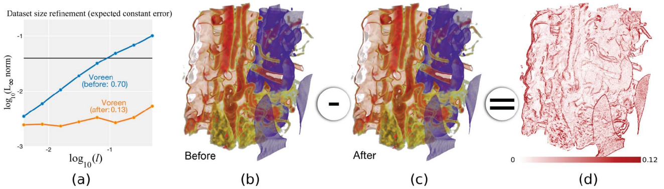
Fig. 1. (a) It shows the result of our verification procedure for data set refinement. The blue line corresponds to the initial behavior, which deviates from the expected slope (solid dark line). After fixing the issues, we obtain the orange curve, with a slope closer to the expected one. (b) and (c) show a human torso, displaying the blood vessels and the spine, before and after our changes. (d) It shows the difference between (b) and (c).
