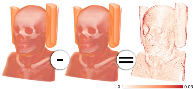
Fig. 2. Left: the volume rendering of the torso data set using an incorrect trilinear interpolation. Middle: Same data set with the correct interpolation. Right: difference between the two images.
