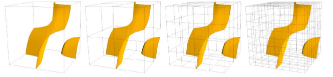
Fig. 5. Isosurface of a randomly generated scalar field defined at different resolutions. The (piecewise) trilinear surface is the same regardless of the grid size.
