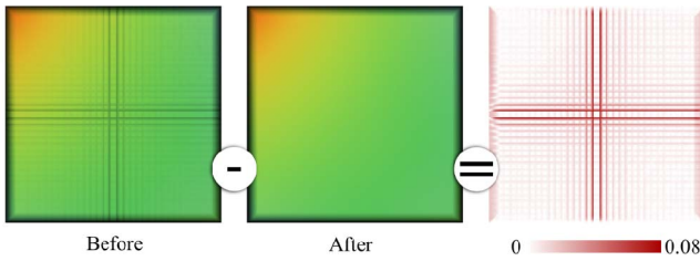
Fig. 8. The figure shows images rendered using VTK 5.6.1. In our experiments, the “+” pattern became more evident in two cases: when coarse data sets are used, and/or high number of sampling points along the ray are used. Darker pixels belong to regions where the ray traverses only half of the volume, preventing convergence. The image on the middle shows the result using our modified version of VTK. The convergence curve improved significantly after the issue was fixed. Note that this effect only occurs when perspective projection is used. For orthogonal projection, the problem is not noticeable. For the convergence analysis, we used a scalar field given by S(x, y, z) = xyz , D = 1 , transfer function \tau(s) = s in the domain [0, 1]^3 , and solution for the VRI given by I(x, y) = 1 - \exp(-xy/2) , which means the integration is along z (from zero to one).
