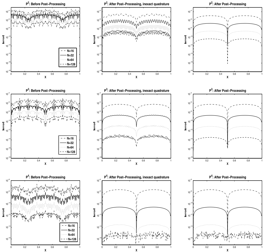
Fig. 1 Point-wise errors on a logarithmic scale before post-processing (left), after post-processing on the consistent integration mesh with inexact quadrature (middle) and after post-processing with exact quadrature (right)
