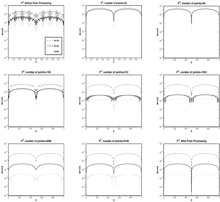
Fig. 5 Point-wise errors on a logarithmic scale when using midpoint integration for post-processing with different number of evaluation points. Top left: before post-processing. Bottom right: after post-processing on the consistent integration mesh
