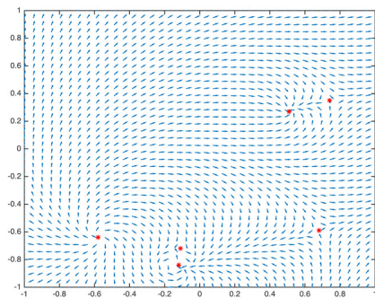
Fig. 12. Synthetic velocity field with known critical points (shown as red dots).
