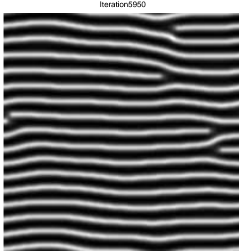
Figure 12: Lines produced by 2D Reaction-Diffusion Process.
