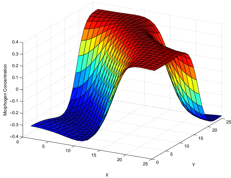
Figure 10: Ermentrout Stripe Pattern Result without Wrap-around Connectivity.
