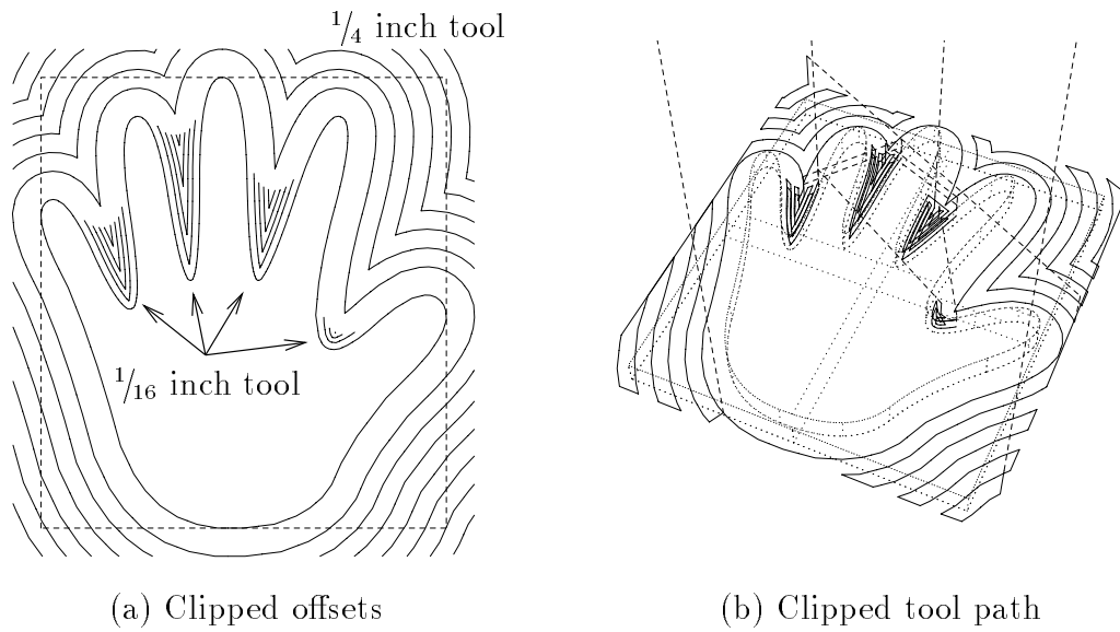
Figure 4.4. Clipped offsets and tool path for multiple tools machining
