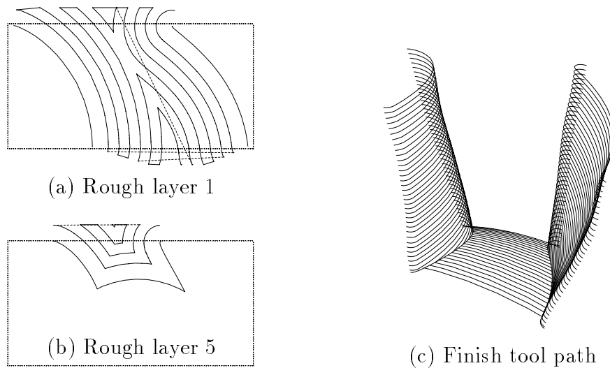
Figure 3.24. Roughing and finish tool paths for a compressor disk
