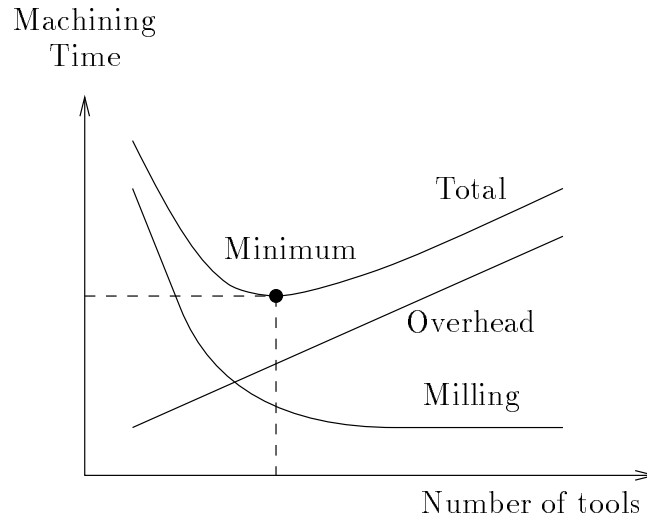
Figure 2.5. Machining time of multiple tools milling operations
