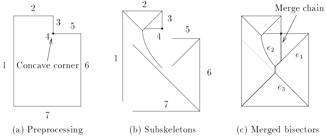
Figure 3.9. A divide-and-conquer merge skeleton algorithm
