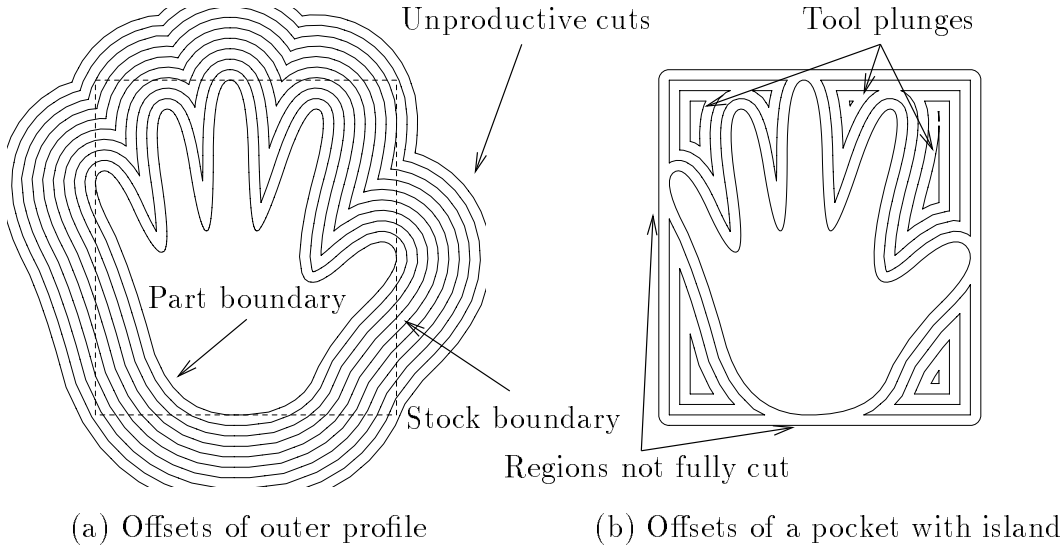
Figure 3.17. Machining of outer profile
