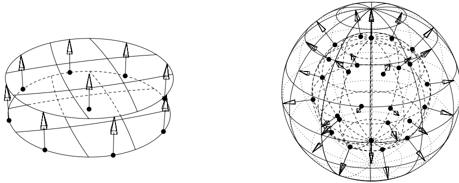
Figure 5.10. Offset interpolation of degenerate surfaces
