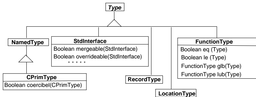
Figure 4: Some concrete type classes
