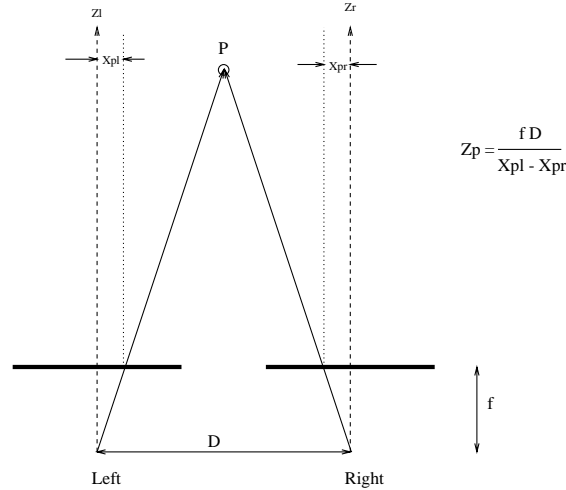
Figure 17: Pinhole Camera Model
