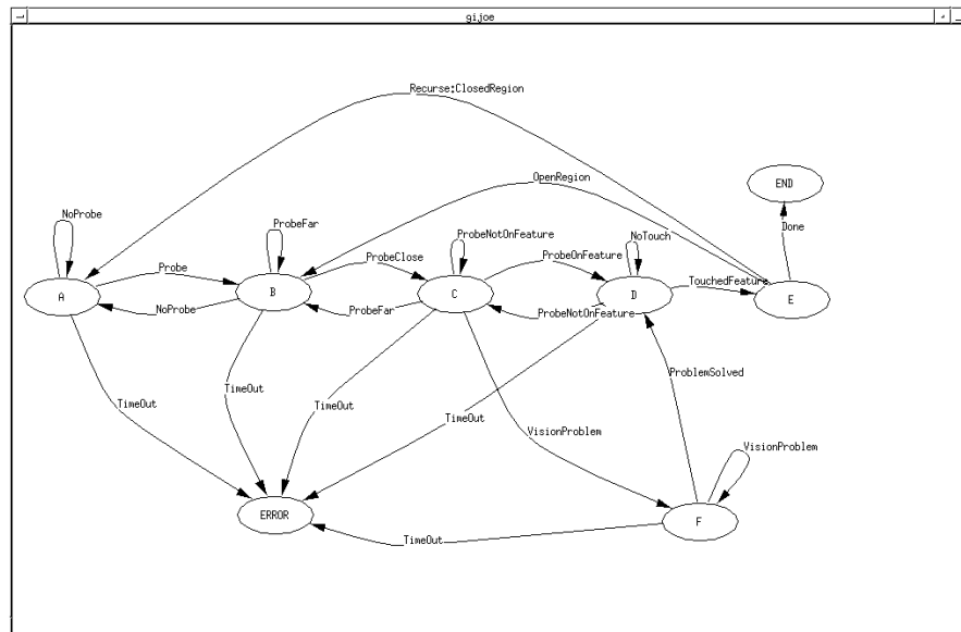
Figure 6: GIJoe Window w/DRFSM
