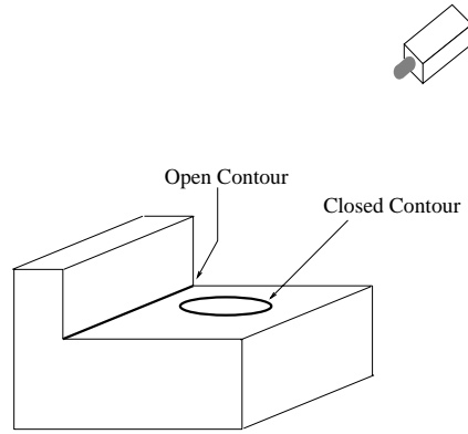
Figure 9: Edge finding in the two dimensional image can give us hints about where to look for three dimensional features. The open contour here is generated where two faces meet. The corresponding contour is then explored by both the stereo layer and the CMM machine.
