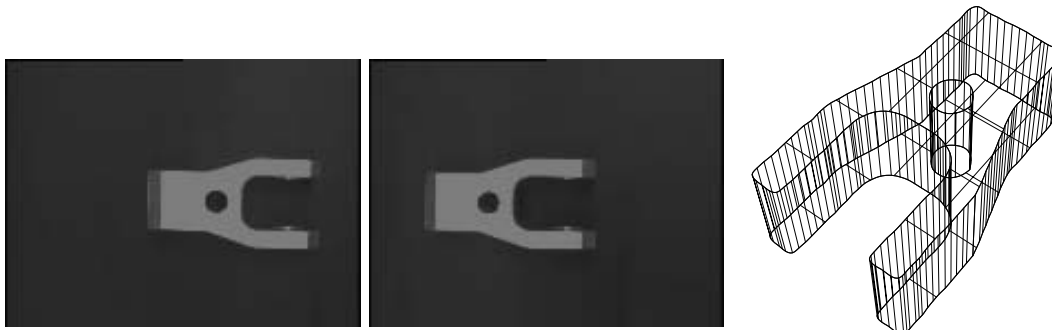
Figure 38: The two stereo images and the final Alpha 1 model that was found in the experiment.
