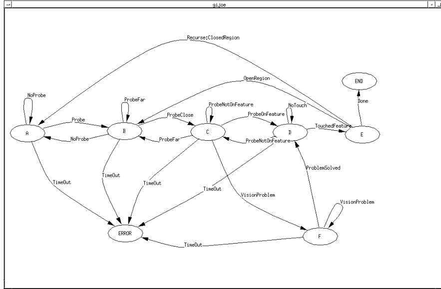
Figure 6: GJJoe Window w/DRFSM
