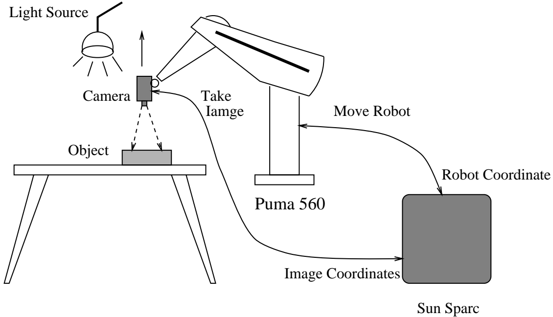
Figure 25: Constructing the Illumination Table off-line
