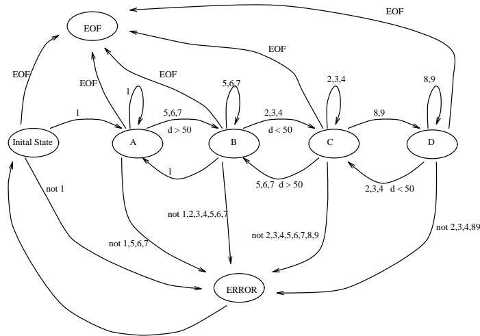
Figure 32: State Machine Used in Test
