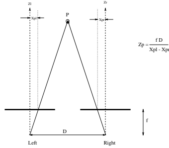
Figure 16: Pinhole Camera Model
