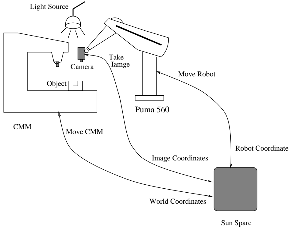
Figure 35: An Experiment For Inspection and Reverse Engineering
