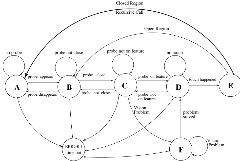
Figure 36: The DRFSM used in the new experiment
