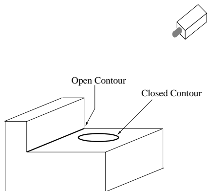
Figure 9: Edge finding in the Two dimensional image can give us hints about where to look for three dimensional features. The open contour here is generated where areas of two different heights meet. The corresponding contour is then explored by both the Stereo layer and the CMM machine.
