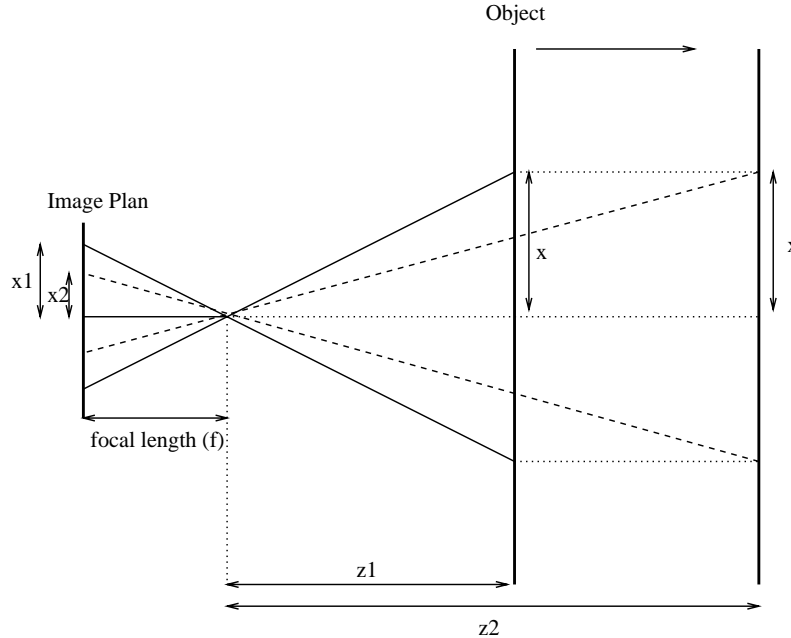
Figure 26: Changing Window Size Assuming Pinhole Camera Model
