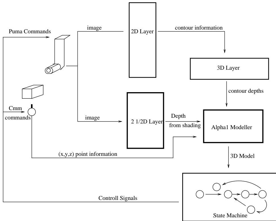
Figure 28: The role of an internal CAD model in the inspection machine
