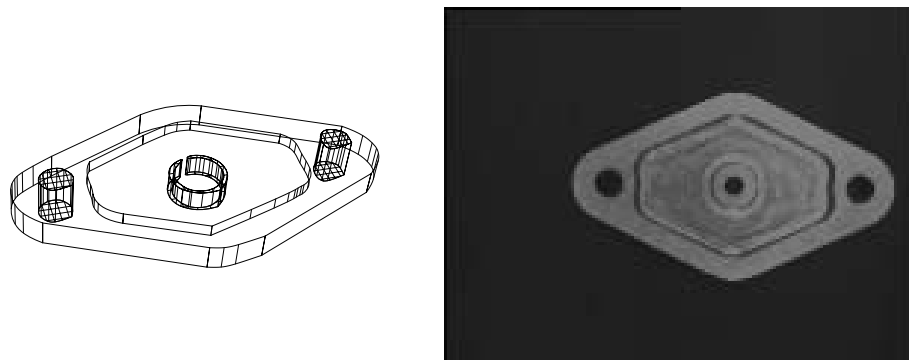
Figure 29: A rough Alpha_1 surface model extracted from the machine vision
