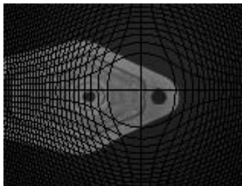
Figure 22: Corrected Image, \kappa = .05
