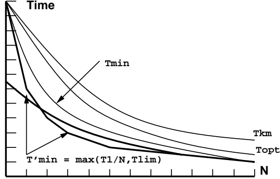
Figure 13: Speedup Graph
